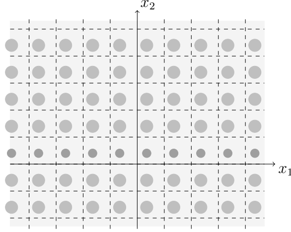
Figure 1: Sketch of a perturbed periodic medium in dimension n = 2 . The medium is characterized by the coefficients of a differential operator. The underlying coefficients, a and b in the guiding example, are periodic in every direction. The perturbation, in the example given by the coefficient q , is confined to a strip \mathbb{R}^{n-1} \times W = \mathbb{R} \times (0, 2\pi) . Our result is that the perturbation reduces spectral gaps of the underlying medium.
