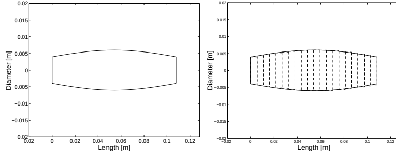
Figure 2: Shape of test rotor and beam element approximation.
