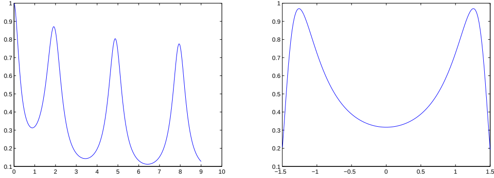
Figure 4: Numerical evaluation of the transmission coefficient |T|^2 . Left: in dependence of the non-dimensional wave-number k for normal incidence, \theta = 0 . Right: in dependence of the angle \theta for wave-number k = 0.8 . In both figures, we used the non-dimensional geometrical quantities \eta = 7/6 , \alpha = 1/7 , and \gamma = (1 - \alpha)/2 = 3/7 as mentioned in (1.7), the frequency independent relative permittivity \varepsilon_\eta = (0.12 + 3.7i)^2 is obtained by setting \sigma = 4.32 - 0.14i .
