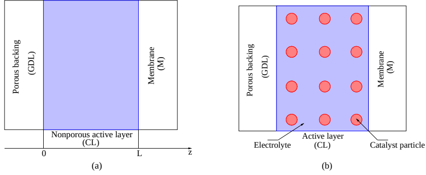
Figure 2: (a) The catalyst layer as a homogeneous meta-material. (b) Catalyst particles included in the electrolyte.
