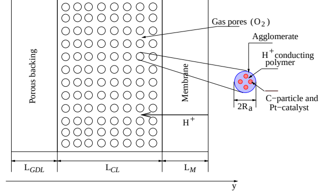
Figure 3: Agglomerates distributed in pore space.
