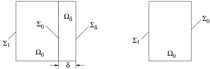
Figure 5: Geometry of the \delta -problem and the effective domain.
