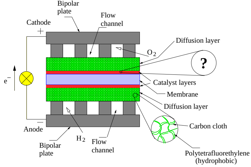
Figure 1: Sketch of a proton exchange membrane (PEM) fuel cell.
