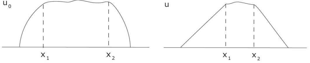
Figure 3: Evolution of the free boundary according to Theorem 2.
