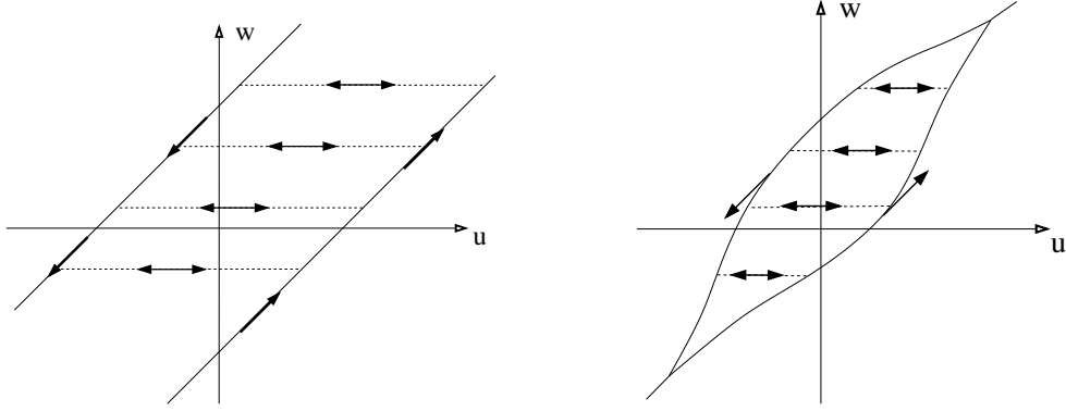
Figure 10: Left: The Play-hysteron. In porous media, u is the pressure and w is the saturation (hence the coordinates are exchanged in comparison to Figure 3). Right: The generalized Play.
