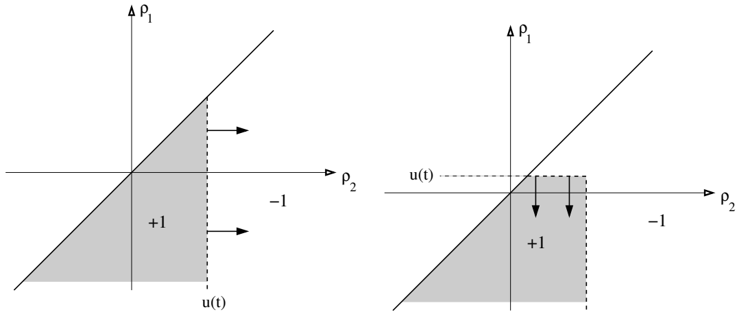
Figure 9: The Preisach plane. Left: An increasing input function u results in flipping all switches along a vertical line at position u(t) . Right: A decreasing input function u results in flipping all switches along a horizontal line at vertical position u(t) .
