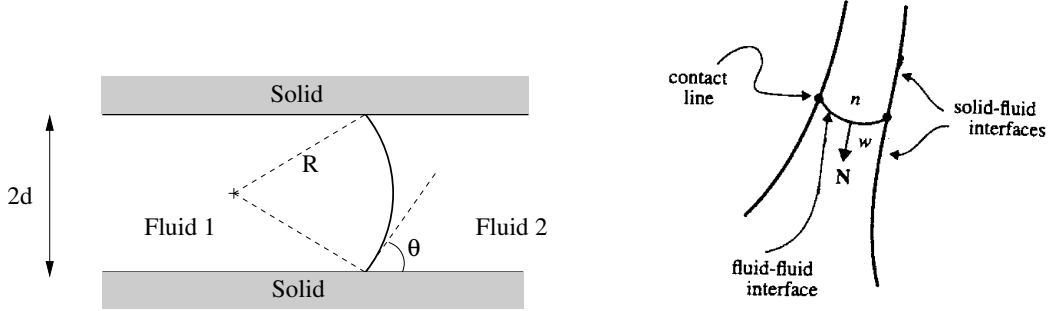
Figure 2: The origin of capillary pressure. Left: A fluid-fluid interface in an idealized pore. The width 2d of the pore together with the contact angle condition determine the curvature 1/R of the meniscus. Right, from [35]: A change in the position of the interface results in a change of the capillary pressure, since the pore diameter changes.
