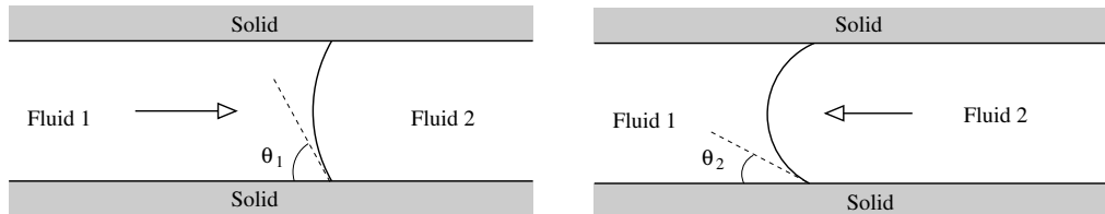
Figure 4: The contact angle is velocity dependent. As a result, the curvature of the meniscus is different for imbibition and for drainage.
