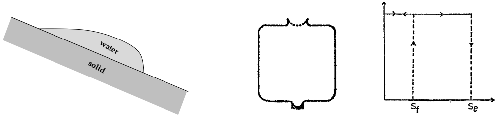
Figure 5: Left: Sketch of a rain-drop, motivating the name “rain-drop effect” for the velocity dependent contact angle. Right: The “bottle-neck effect” in an illustration from [75] with a classical ink-bottle. The ink-bottle acts as a relay: it takes a high suction S_e to empty the ink-bottle and a lower suction S_f to fill the ink-bottle (note that the suction is |p| , the positive difference of water levels).
