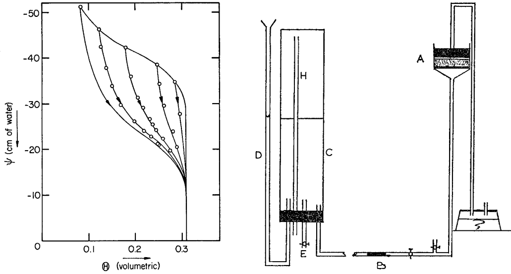
Figure 3: Left: From Mualem [62]. Capillary pressure curves or “water retention curves”. We note that in a more natural representation (flipping the vertical axis), all curves of the diagram (water pressure against water saturation) are monotonically increasing. Right: From Poulouvassilis [75]. Apparatus for the measurement of the capillary head.
