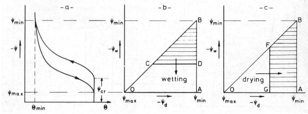
Figure 8: Active regions for various switches from Mualem [60]. In b and c, the horizontal coordinate axis is -\Psi_d , the pressure value at which drainage occurs (the upper switching value). The vertical coordinate axis is the wetting pressure -\Psi_w (the lower switching value). In a wetting process, a horizontal line moves downward (the height is the macroscopic pressure at every time instance), all switches above the line are flipped (the pores are filled). In a drying process, a vertical line moves right (the horizontal position is the macroscopic pressure at every time instance), all switches left of the line are flipped (the pores are emptied).
