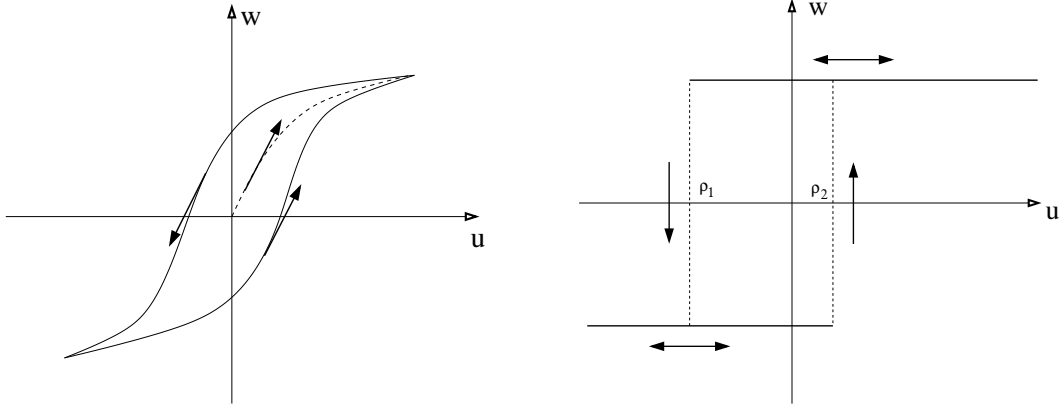
Figure 1: Left: A hysteresis loop. An increasing input u results in an increasing output w , and a decreasing u results in a decreasing w . But the changes of w lag behind those of u . Right: The Relay hysteron, a switch with delay. The Relay shares qualitative properties with the hysteresis loop. It can be used as a building block for more complex hysteresis effects.
