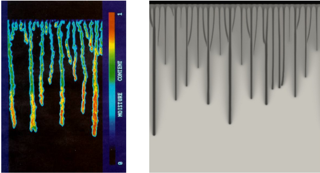
Figure 11: Left: An experimental result for fingering in a porous medium (courtesy of R.J. Glass of the Soil and Water Laboratory at Cornell). Right: Numerical solution of a model with hysteresis and dynamic effect [78].
