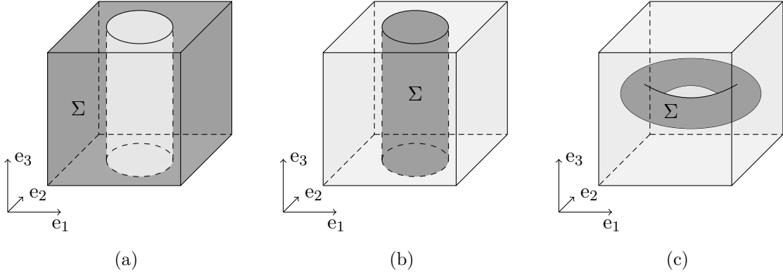
Figure 4: The periodicity cell Y is represented by the cube. (a) The air cylinder Y \setminus \overline{\Sigma} of Example 5.3 (b) The metal cylinder \Sigma of Example 5.4. (c) \Sigma is a 2-dimensional full torus. In this case, Y \setminus \overline{\Sigma} is not a simple Helmholtz domain.
