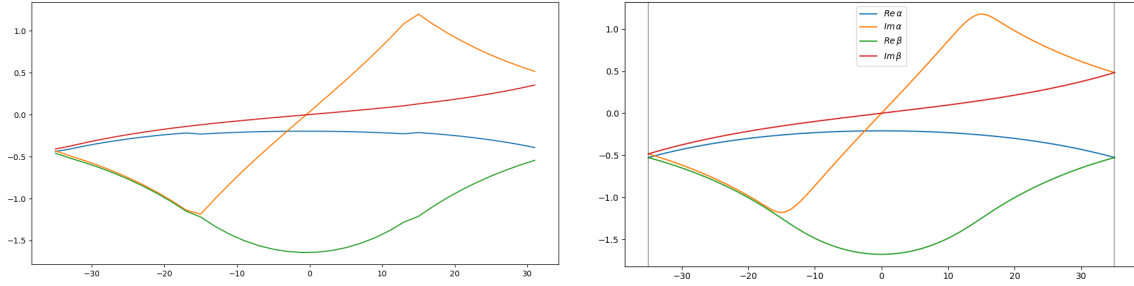
Figure 8: Factors \alpha and \beta for Medium I, r_0 = 0.25 + 0.03 . Left: A two-dimensional calculation for \lambda = 8.07 . For the solution u of (3.1) we plot, for integers r \in (-35, 35) on the horizontal axis, the real and imaginary parts of the integrals \alpha_{\text{num}}(r) = \int_{Q_r} u \bar{V} and \beta_{\text{num}}(r) = \int_{Q_r} u \bar{W} . The curve with the highest maximum is \text{Im}(\alpha) , the curve with the lowest minimum is \text{Re}(\beta) , the monotonically increasing curve is \text{Im}(\beta) . Right: Solutions of (3.4)–(3.5) with A = 1/(2\pi) , p = 0 and q = 0.045 .
