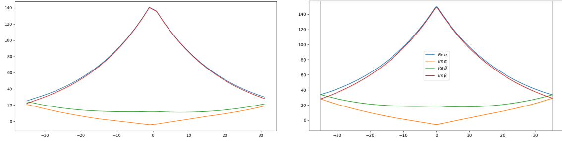
Figure 11: Solutions in the combined medium, Medium I for x_1 > 0 and Medium II for x_1 < 0 . Left: 2D calculation for \lambda = 8.05 . Right: System (3.4)–(3.5) with q = 0.045 for x > 0 , q = -0.045 for x < 0 and p = -0.0005 . We observe that the qualitative features of the solution are well predicted by the ansatz (4.6) with a large real constant B (the two functions with the high maximum in t = 0 are \text{Re}(\alpha) and \text{Im}(\beta) ).
