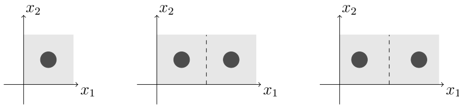
Figure 3: Left: The cell (0, 1/2) \times \Sigma corresponding to media with 1/2 -periodicity. Middle: The same medium, now regarded as 1-periodic with the periodicity cell (0, 1) \times \Sigma . Right: A perturbation of the 1-periodic medium cell leads to a 1-periodic medium that is no longer 1/2 -periodic.
